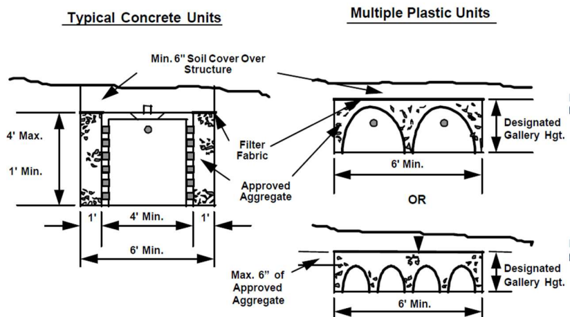
Figure 15. Typical Leaching Gallery Structures
