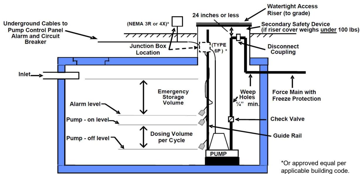
Figure 10. Pump Chamber
