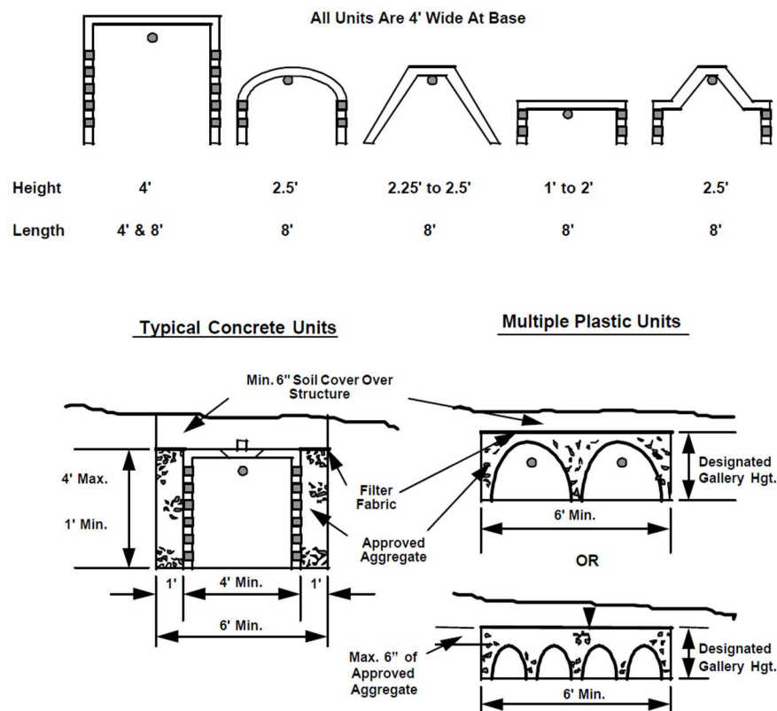
Figure 15. Typical Leaching Gallery Structures
