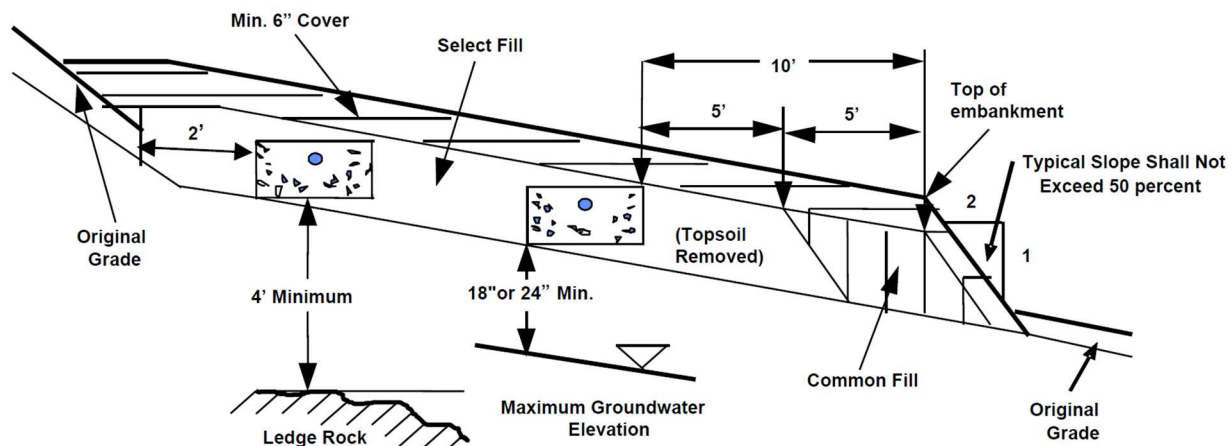
Figure 12. Minimum Separating Distances Above Ledge Rock and Maximum Groundwater
