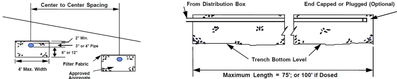
Figure 13. Leaching Trenches
