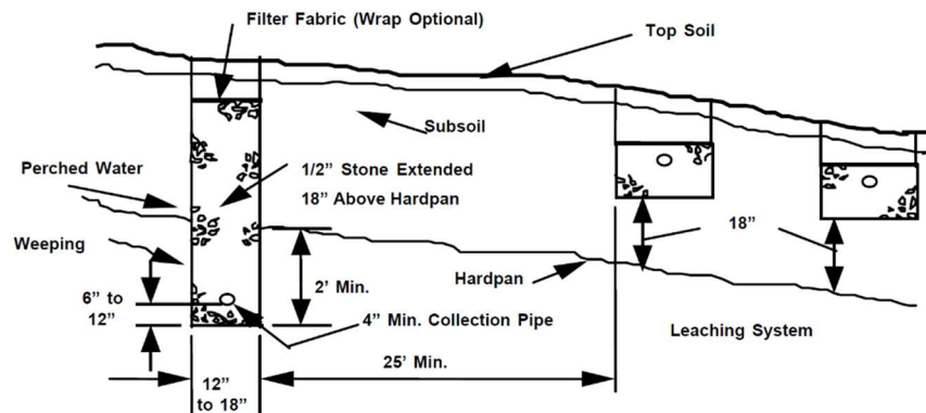
Figure 16. Typical Curtain Drain Construction
