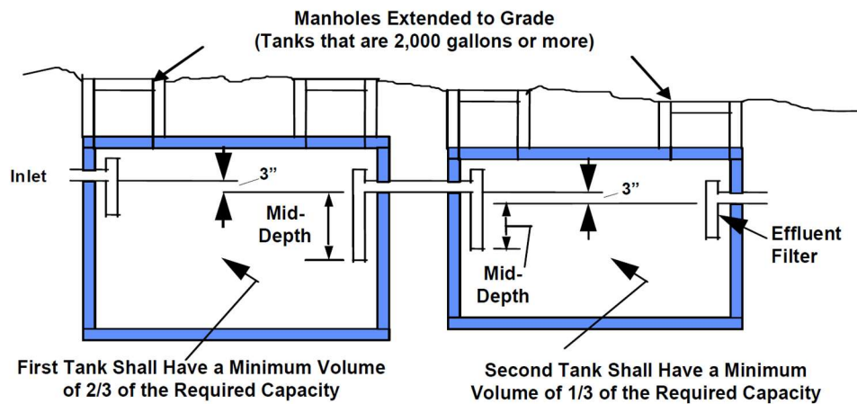
Figure 4. Two Septic Tanks in Series
