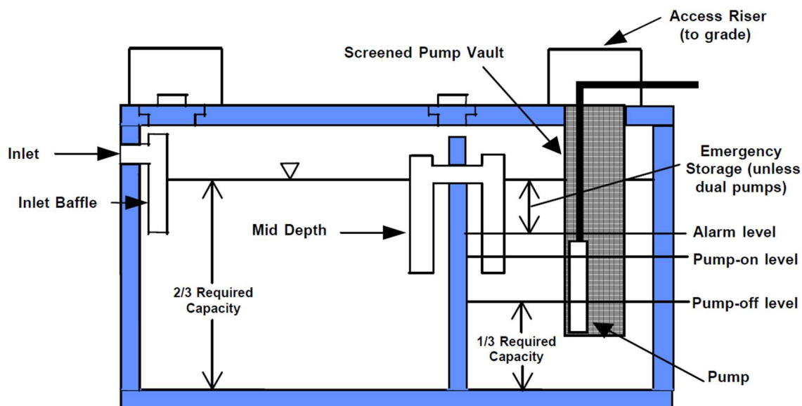
Figure 11. Combination Septic Tank/Pump System with Tee Baffle Connection
