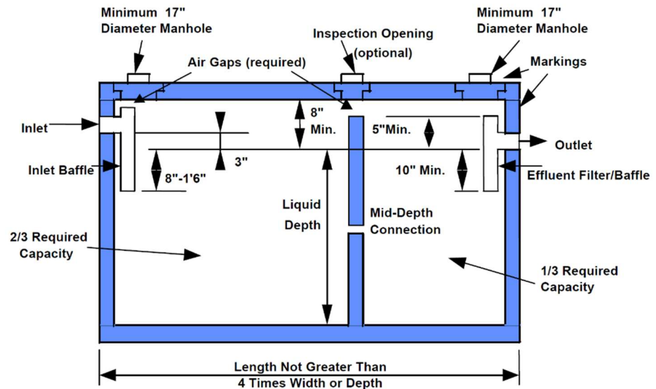
Figure 3. Typical Septic Tank Configuration
