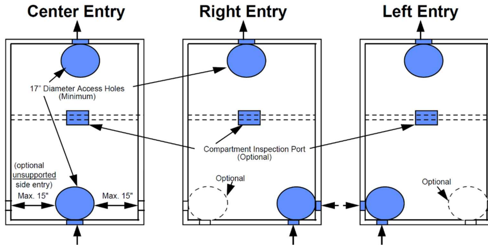
Figure 5. Standard Septic Tank Configurations
