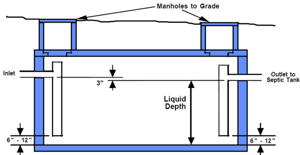
Figure 6. Grease Interceptor Tank (GIT)
