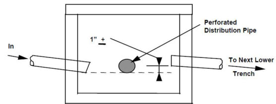
Reversed Distribution Box
