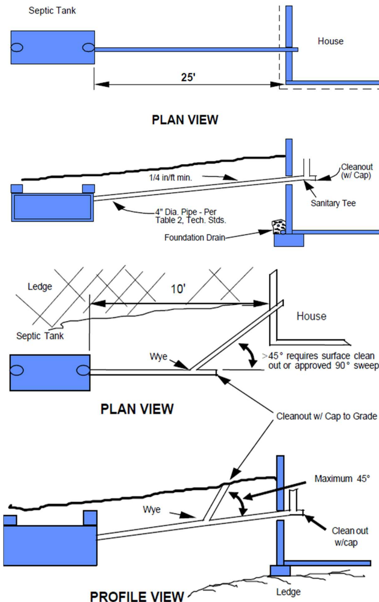
Figure 1. Building Sewers
