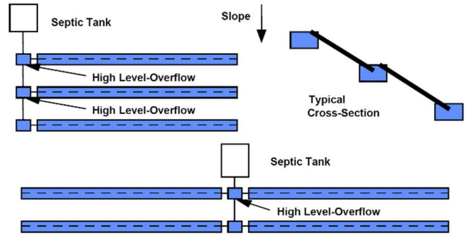
Figure 8. Serial Distribution Systems
