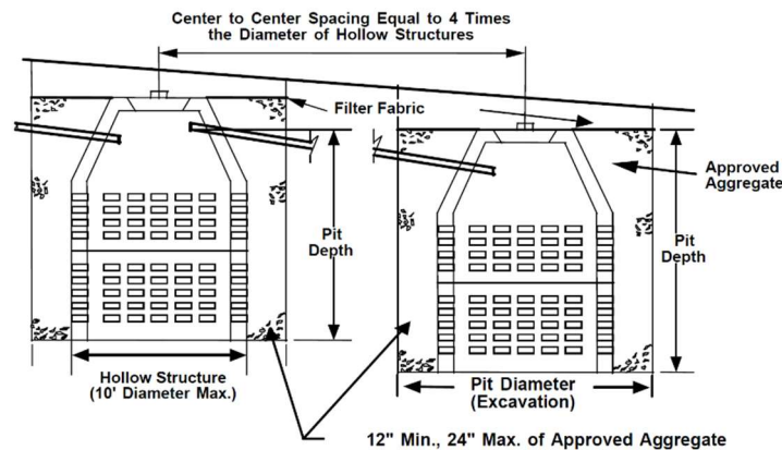
Figure 14. Leaching Pits
