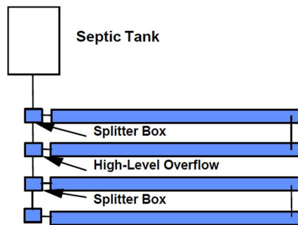
Figure 9. Alternative Distribution Systems and D-Box Configurations
