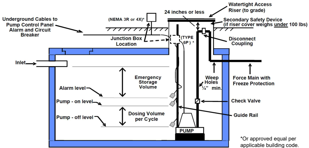
Figure 10. Pump Chamber
